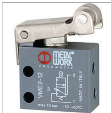
3/2-Wege Ventil NO 3/2-Way valve N.O.
